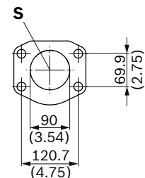
Detail W
