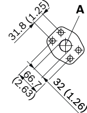
Detail Z
