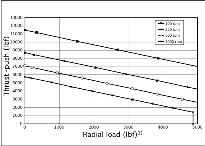
Combined load at 3000 hrs L 10 bearing life
