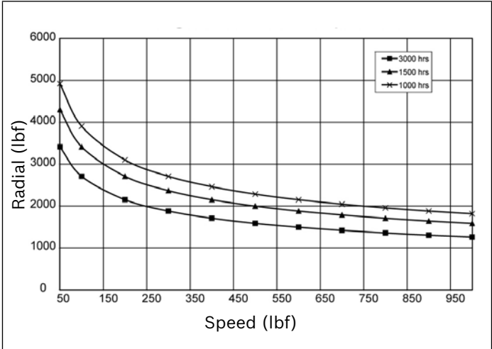
Bearing load at center of output shaft
